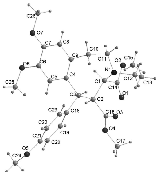
Figure 1. X-ray crystal structure of 47 .
